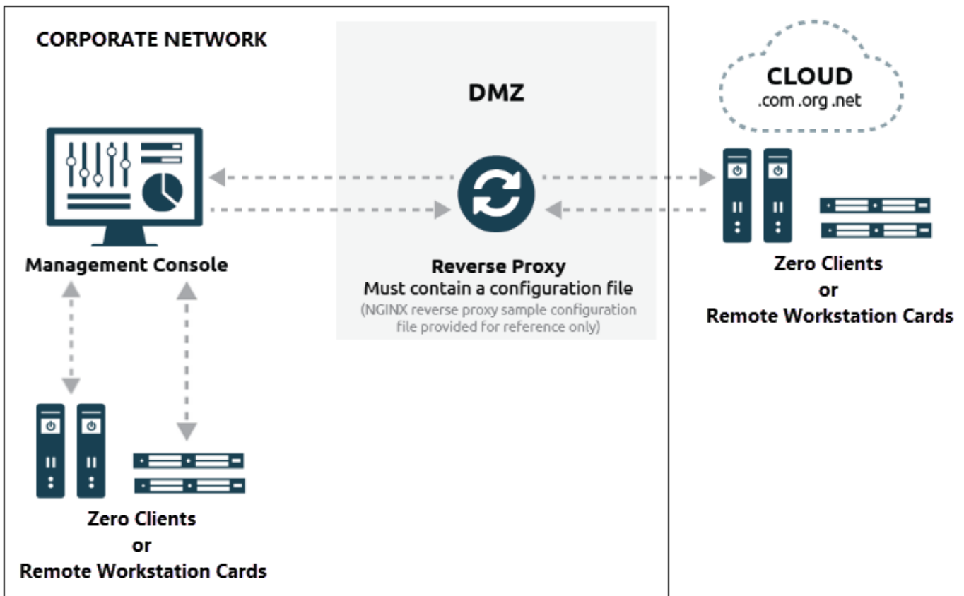
Reverse Proxy Configuration
